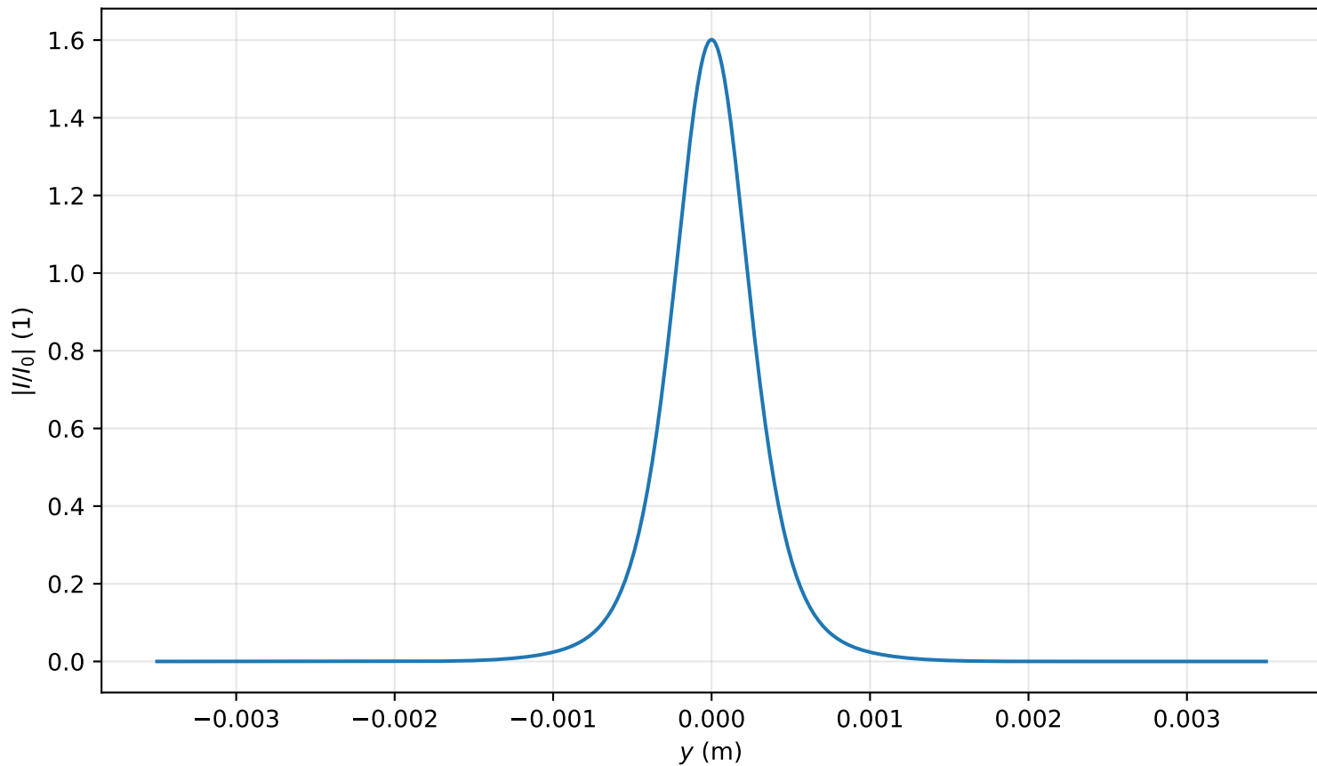
Intensity profile I(x=0, y, z=1.672)/I_0 , P_{in}=0.9P_{cr} , artificial time
